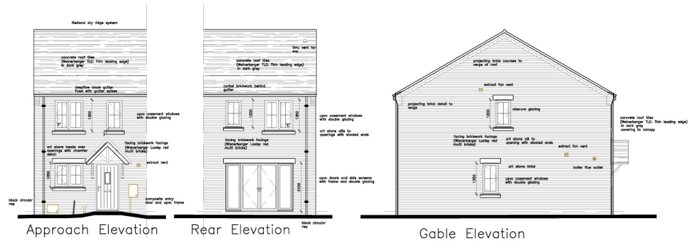
Gable Elevation
